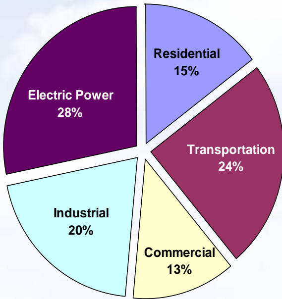
Domestic CO 2 Emissions by Sector (2006)
