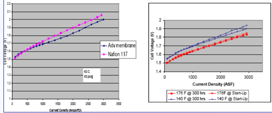
Demonstration of Advanced Membrane in 160-cm 2 cell
