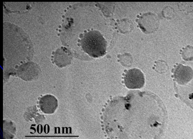
fs-laser irradiated soda-lime glass
