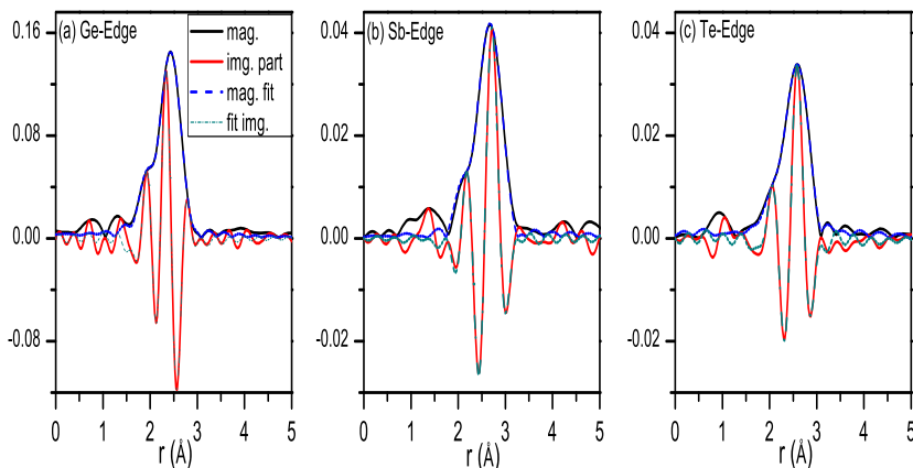
Atomic structure of electrodeposited \text{a-Ge}_2\text{Sb}_2\text{Te}_5 measured by extended X-ray absorption fine structure
