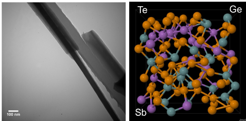
Left: TEM image of amorphous phase-change nanowire Right: Simulated atomic structure of amorphous \text{Ge}_2\text{Sb}_2\text{Te}_5
