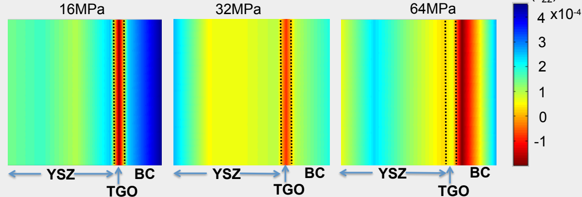
In Plane Strain for the High Temp Point
