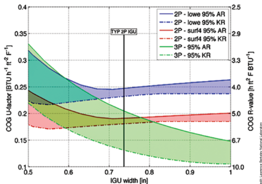
Figure 4. Thermal performance of double glazing (2P) compared to triple glazing (3P) windows at various insulating glass unit (IGU) thickness and filled with argon (AR) or krypton (KR). Blue represents most windows currently on the market. Red represents windows with an additional low-E coating on the inside surface, indicating modest performance gains. Green indicates significant potential energy savings with triple-glazed units.
